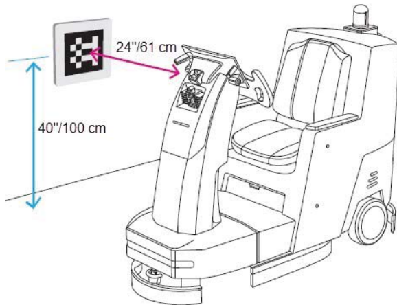
Figure 26: Home Marker distance and height measurements
